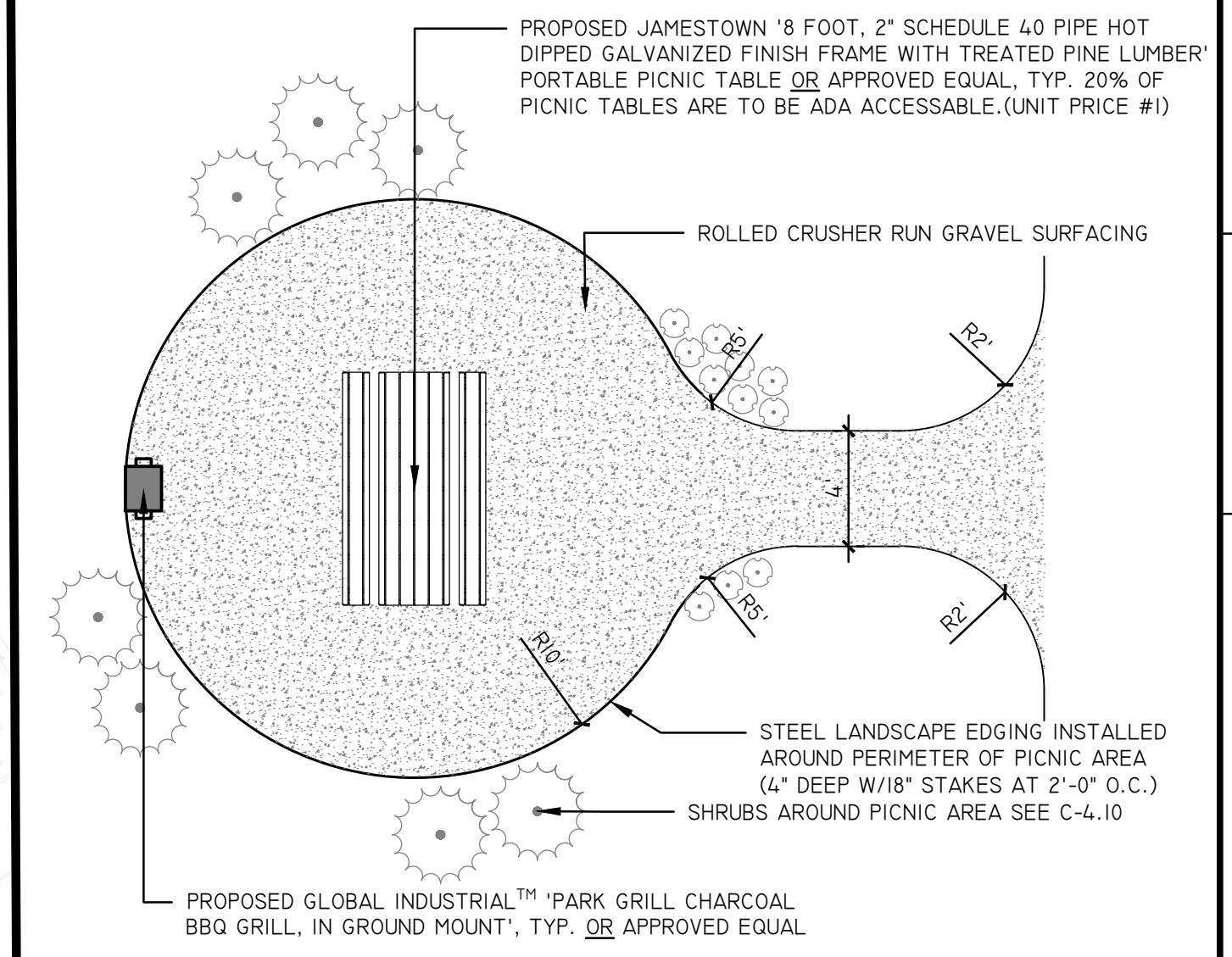
4 TYPICAL LAKESIDE PICNIC AREA DETAIL SCALE: 3/16"=1'-0"
