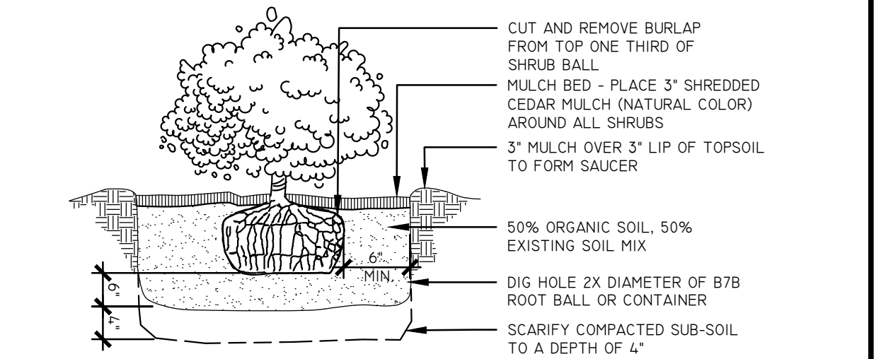
3 BALLED & BURLAPPED (B&B) DETAIL SCALE: N.T.S.
